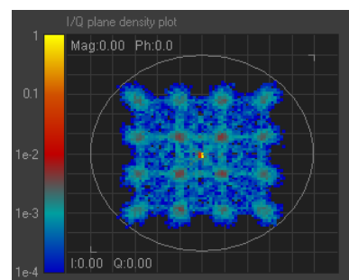
Fig. 44: I/Q density plot
