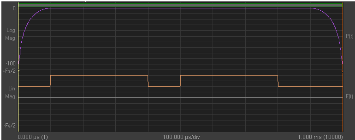
Fig. 26: FSK modulated signal
