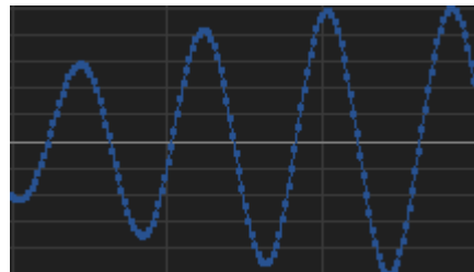
Fig. 37: Zoomed in
