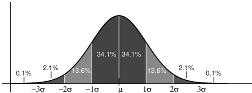
Fig. 13: Normal Distribution
