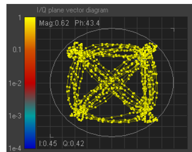
Fig. 43: I/Q vector diagram
