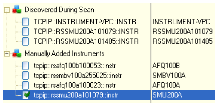
Fig. 3: Instrument selection
