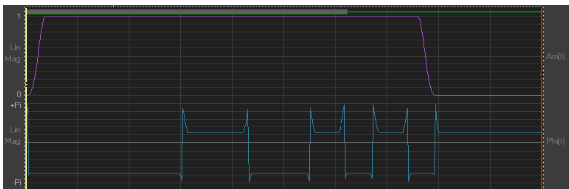
Fig. 39: Polar view of a BPSK modulated signal
