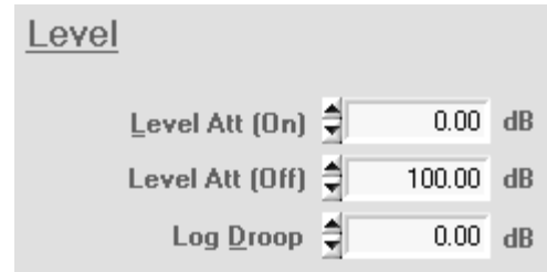
Fig. 8: Level settings
