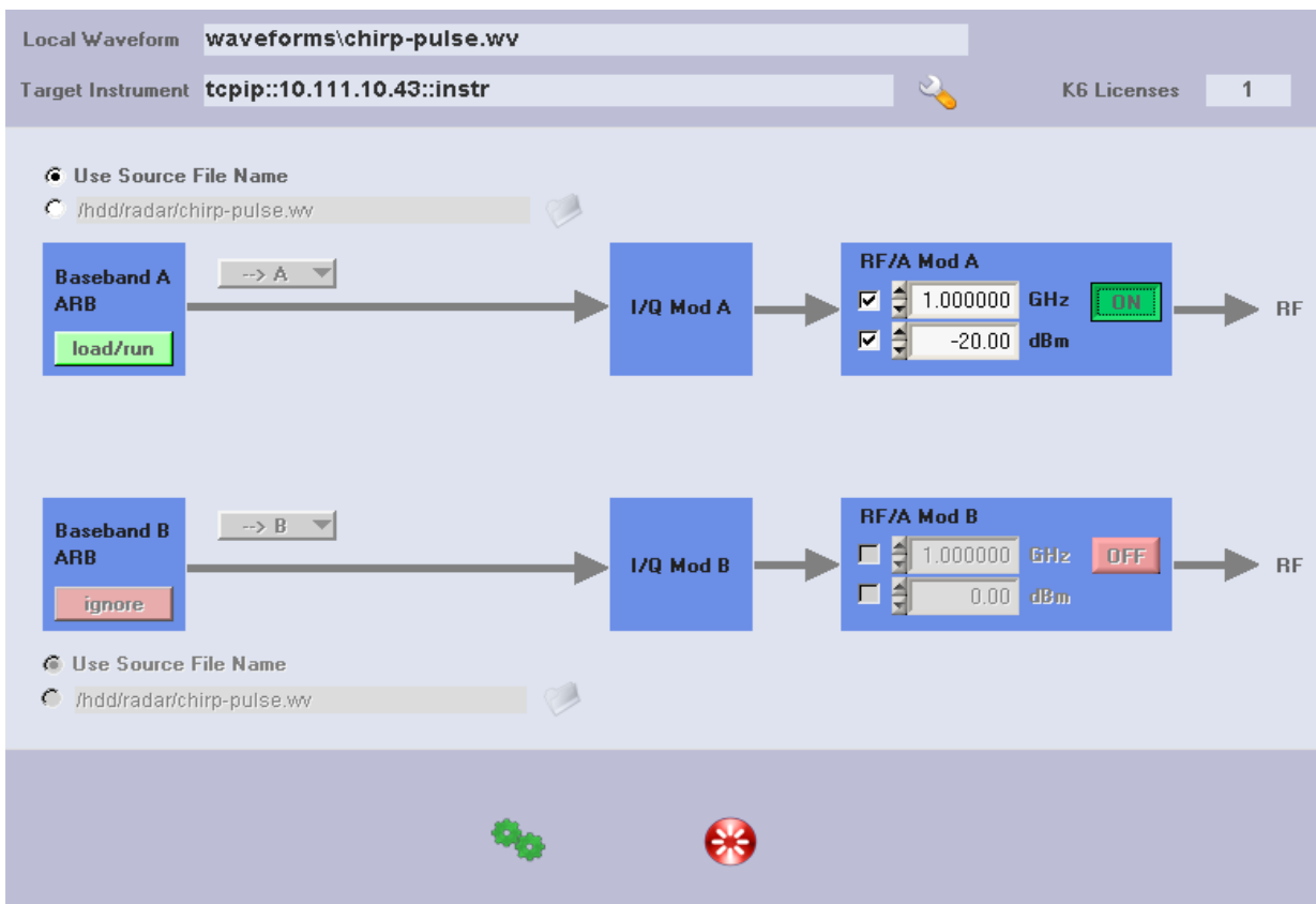
Fig. 46: Transfer panel
