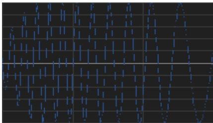
Fig. 36: Zoomed out
