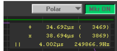
Fig. 42: Marker controls
