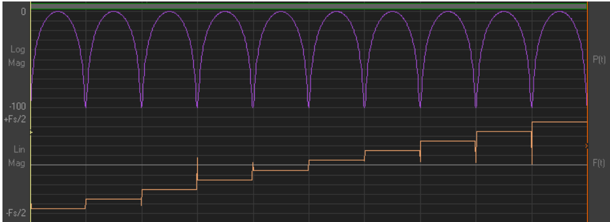
Fig. 14: Example for pulse frequency affected by linear ramp jitter
